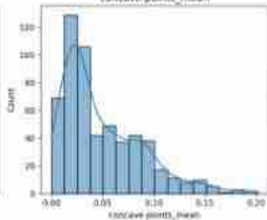
concave points_mean
