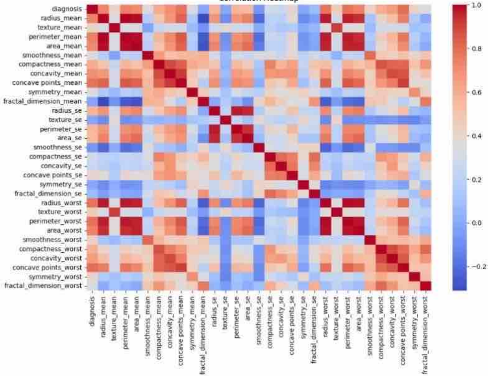
Correlation Heatmap
