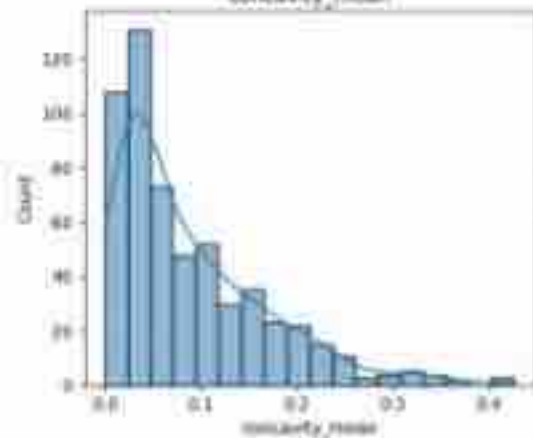
concavity_mean
